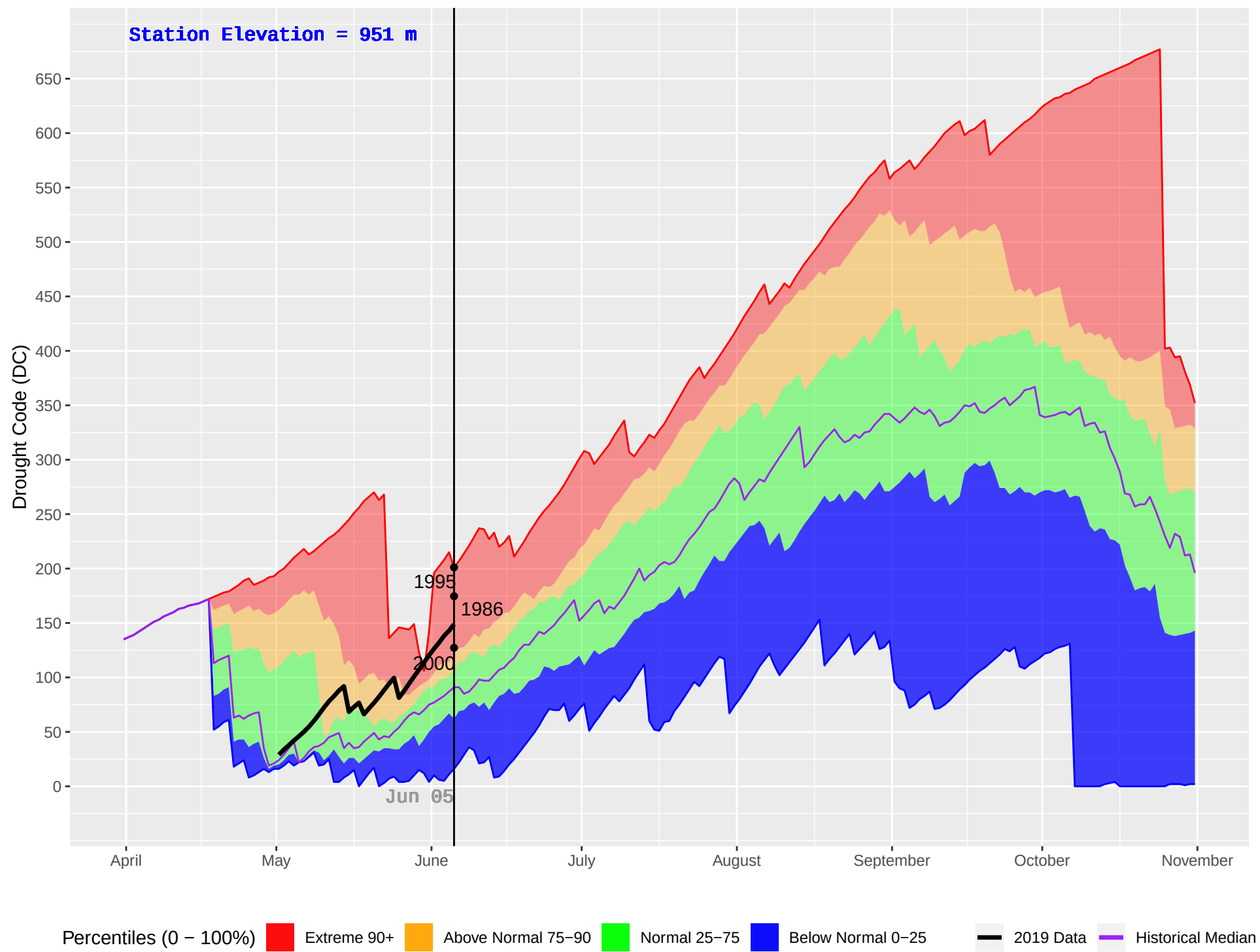
NORTH BABINE (173) : Historical (1986–2018) and Current (2019) Daily Drought Code (DC)
