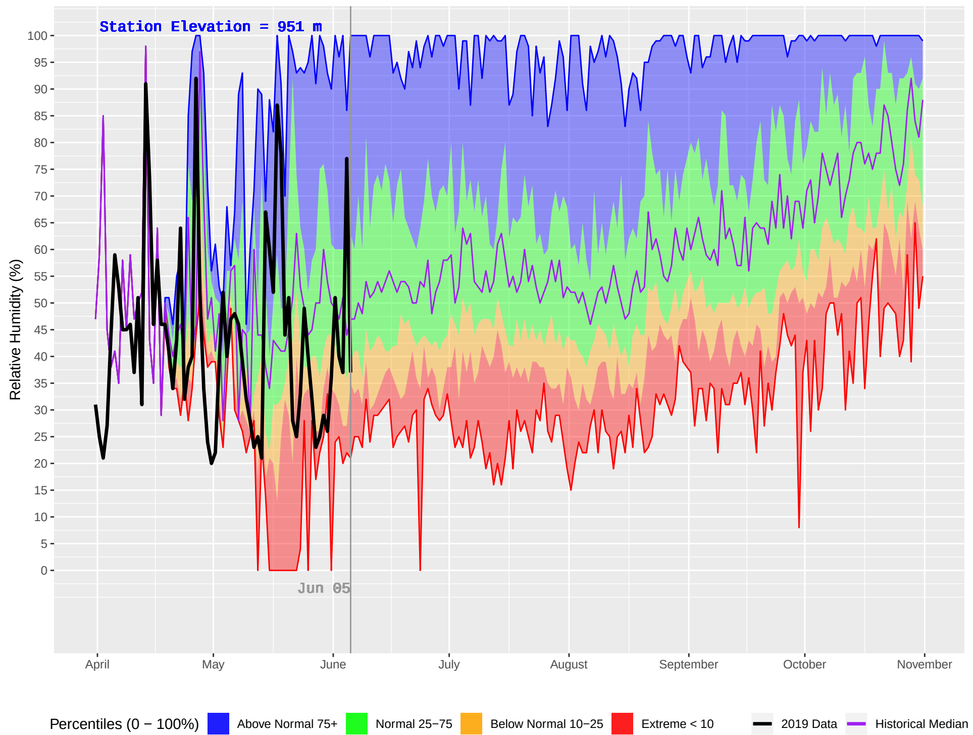
NORTH BABINE (173) : Historical (1986–2018) and Current (2019) Daily Relative Humidity
