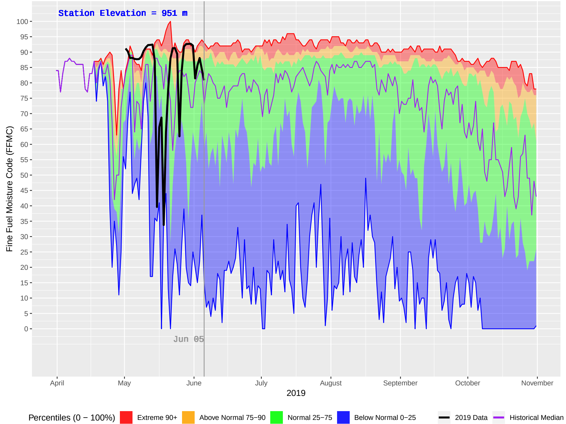
NORTH BABINE (173) : Historical (1986–2018) and Current (2019) Daily Fine Fuel Moisture Code (FFMC)
