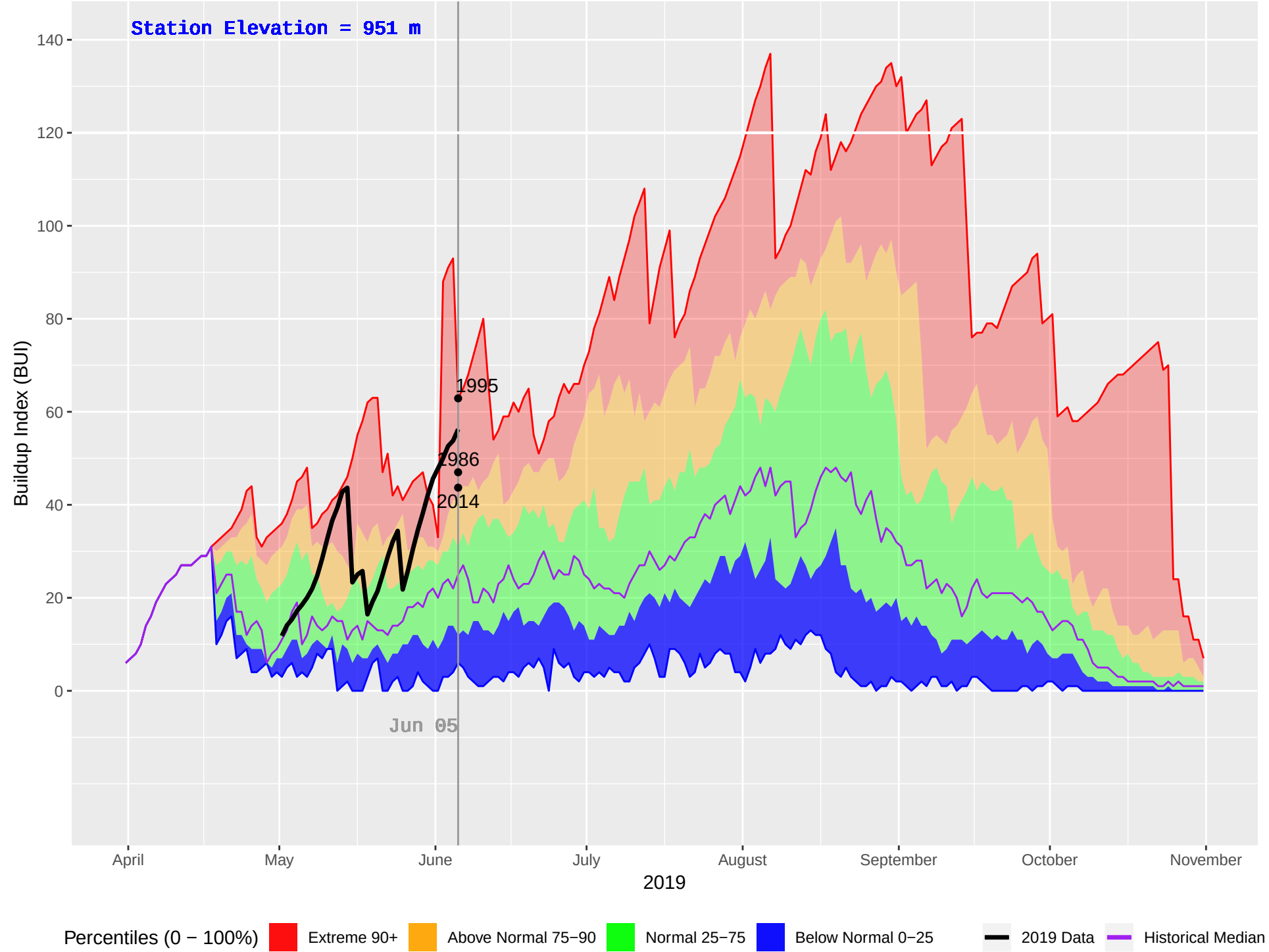
NORTH BABINE (173) : Historical (1986–2018), Current (2019) Daily Buildup Index (BUI)
