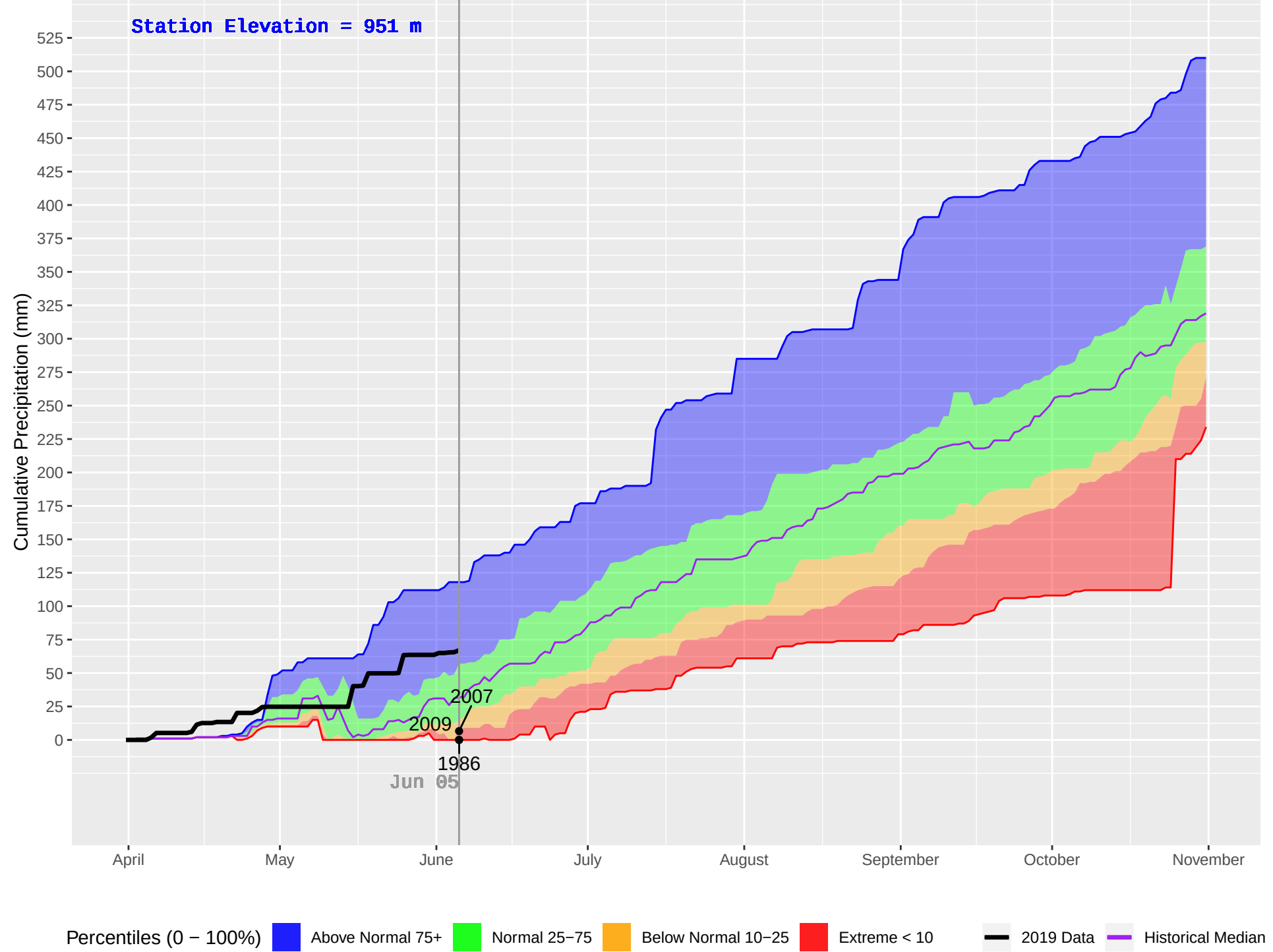
NORTH BABINE (173) : Historical (1986–2018), Current (2019) Daily Cumulative Precipitation
