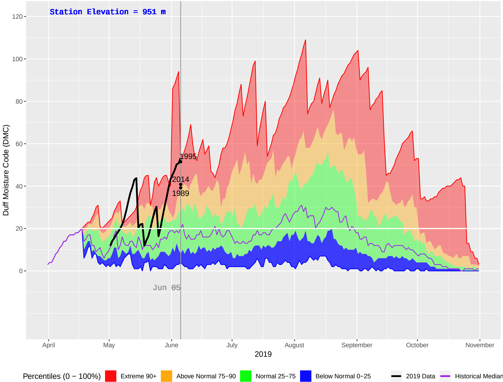
NORTH BABINE (173) : Historical (1986–2018), Current (2019) Daily Duff Moisture Code (DMC)
